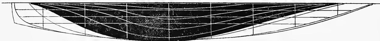
THE SWEDISH RACING SCHOONER YACHT SVERIDGE.
